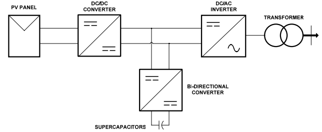
Fig. 5. Supercapacitor in an electrical microgrid
