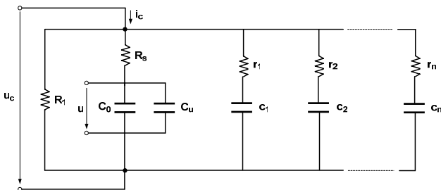
Fig. 4. Model of a supercapacitor
