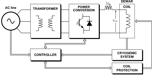
Fig. 3. Superconducting magnetic energy storage system
